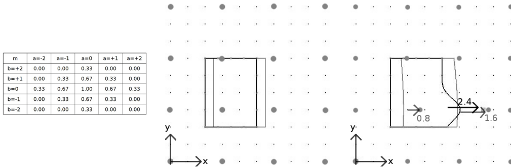
Figure 4. a) Table of multiplier values m_{i,j} , b) Initial top and bottom layer rectangle, c) Coupled deformation of top and bottom layer geometry by manual repositioning of control point P,T_{5,3}
