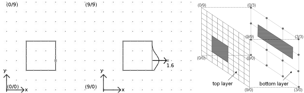
Figure 3. a) A square embedded in a standard FFD control volume, b) deformation of a square by FFD, c) realization of dynamic FFD by coupling a top and bottom layer control point grid
