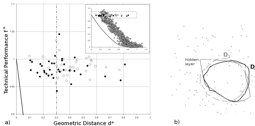
Figure 7. a) Summary of experimental results, b) Computationally optimized shape D4 (fd4=0.35)
